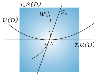
Figure 2: The submanifolds \mathcal{W}_N^s
