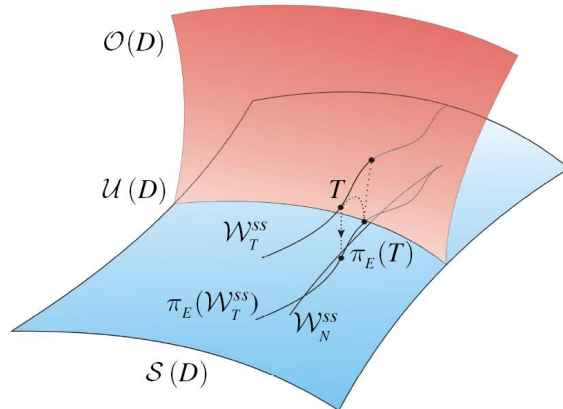
Figure 3: The projection argument
